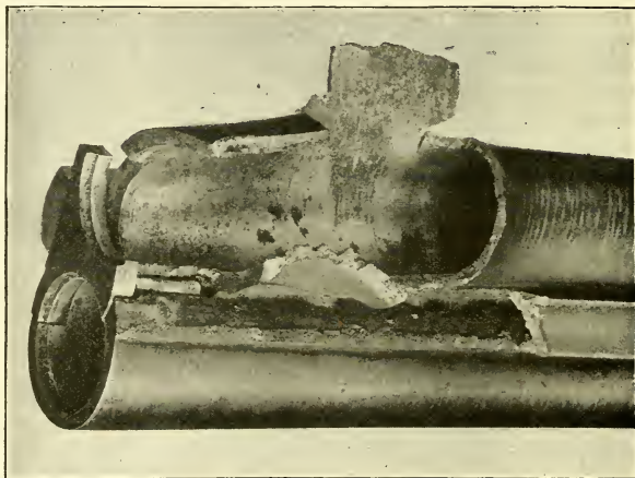
Barrel Burst with Quick-burning Nitro.
